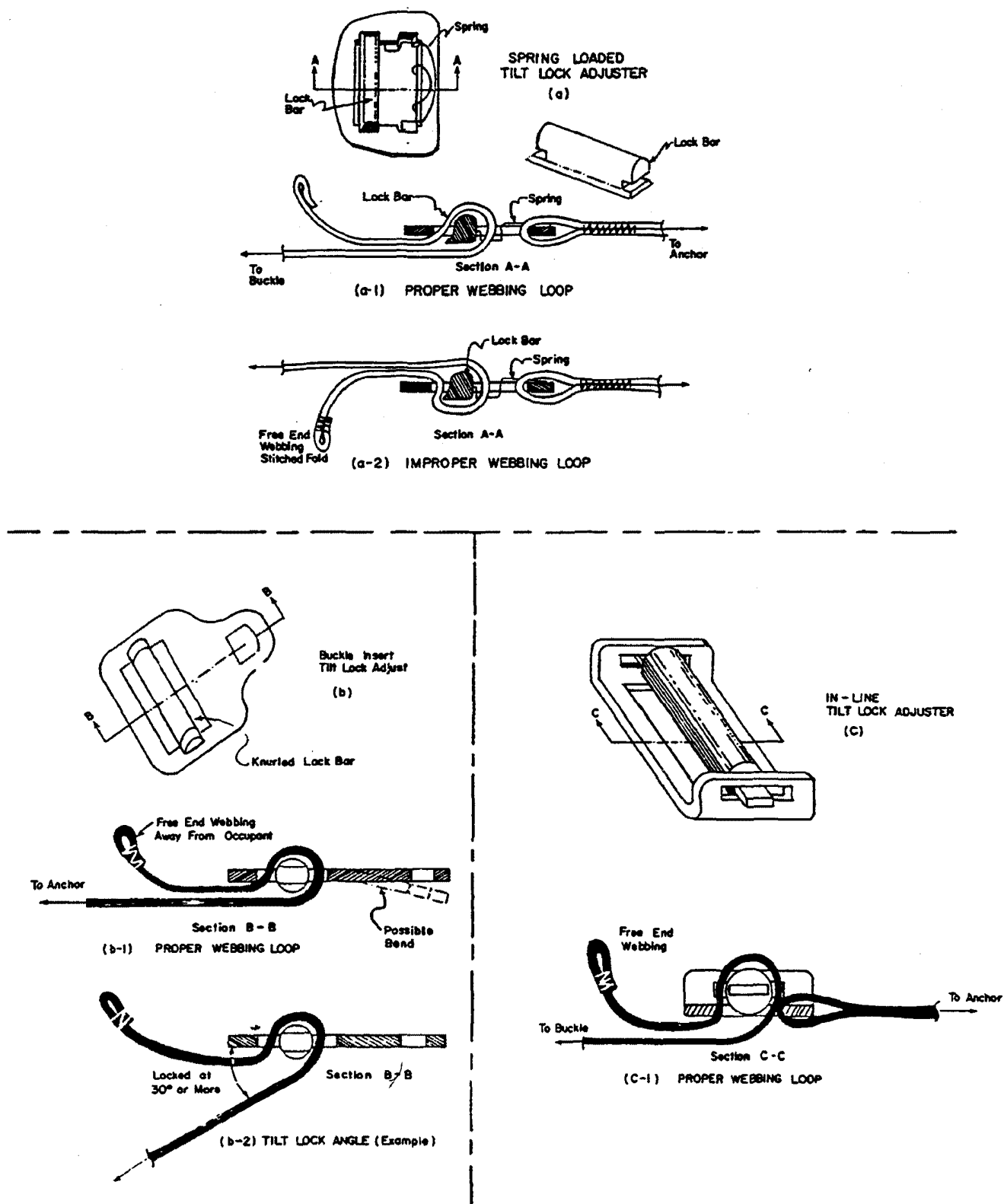
Figure 6. Tilt Lock Adjuster Webbing Loop
